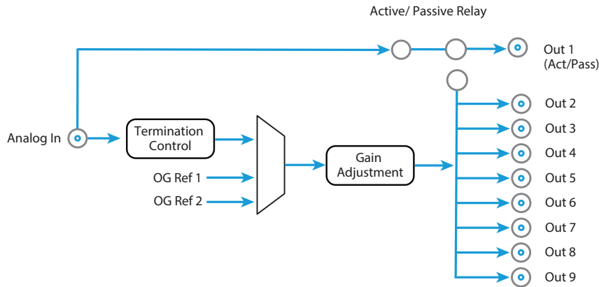
Figure 1. OG-C10DA Converter, Simplified Block Diagram
