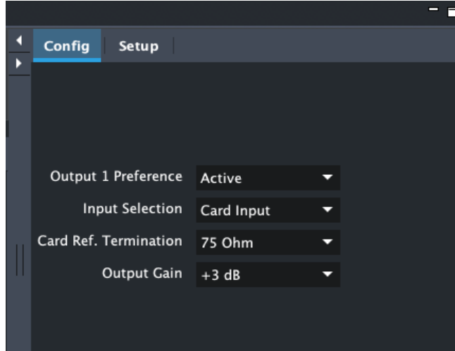
Figure 13. OG-C10DA Config Tab Screen in Dashboard
