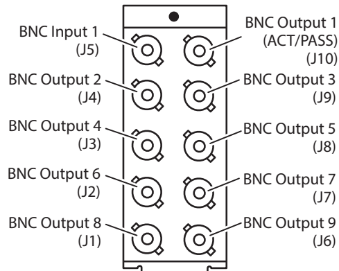
Figure 2. OG-C10DA Converter Connections
