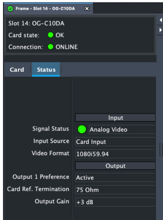
Figure 12. OG-C10DA Status Tab Screen in Dashboard
