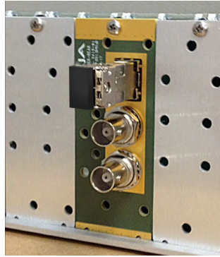
Figure 9. Fiber SFP Installation
