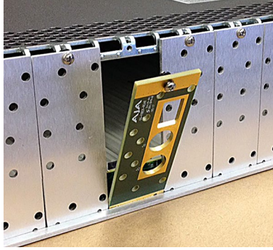
Figure 5. Rear Card Inserted into Frame Seating Slot
