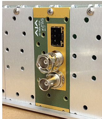
Figure 8. BNC Star Washer and Nut Installation
