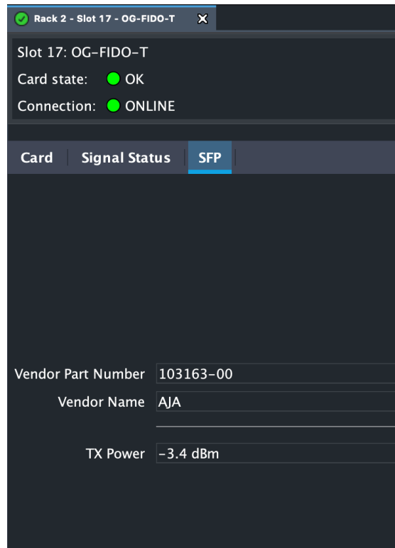
Figure 14. SFP Tab Screen in Dashboard
