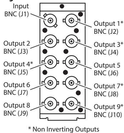
Figure 1. Rear View of Rear BNC Card
