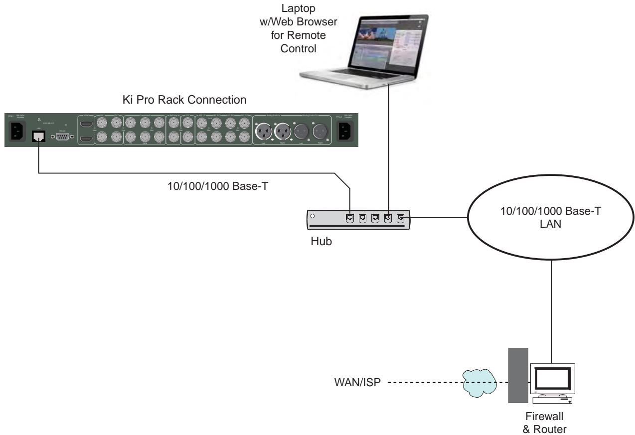
Figure 5. Ki Pro Networking Example
